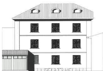
Alzado interior
